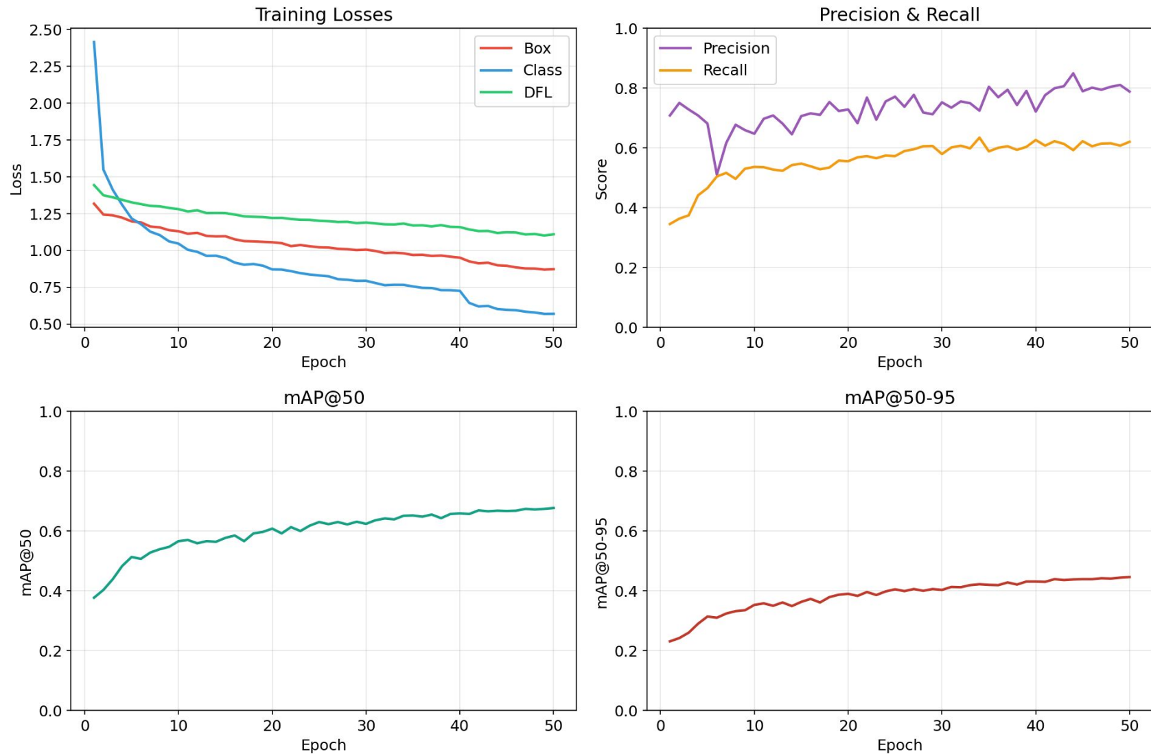
YOLOv8n PPE Detection - Training Metrics Dashboard (50 epochs)
